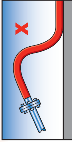
NEVER USE HOSE UNSUPPORTED
