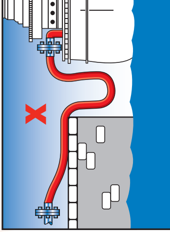
NEVER OVERBEND HOSE OR ALLOW HOSE TO HANG BETWEEN QUAY AND SHIP
