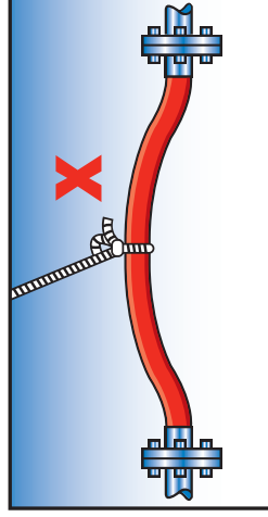
NEVER SUPPORT HOSE WITH SINGLE ROPE
